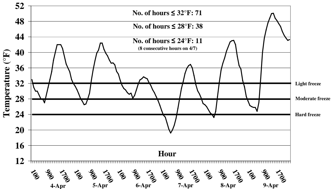
Average Hourly Temperature at Columbia, MO (April 4-9, 2007)
